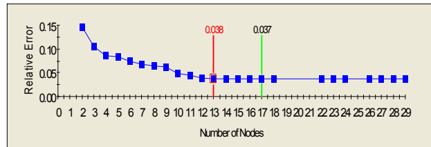
Fig. 3 Diagram of the relative errors of CART models for a linear model with 10 predictors
