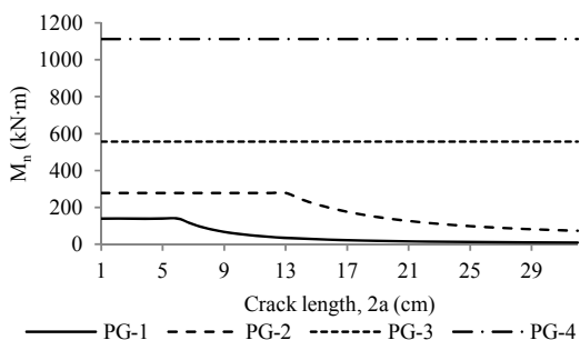
Fig. 9 Bending moment capacities of PG-1 through PG-4 web plates plotted as functions of crack length
