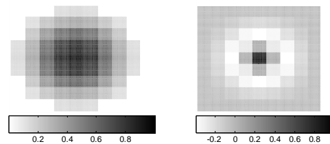
Fig. 8 Spline disk wavelets for segmentation, left: D_1 , right: D_2
