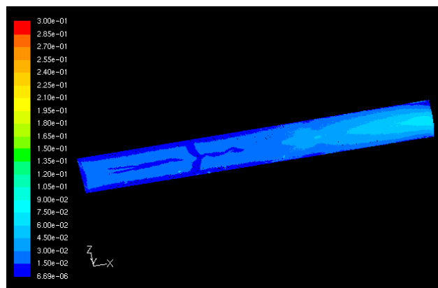
Fig. 8 Velocity distribution on the screen surface facing to the channel for different cases of flow rates
