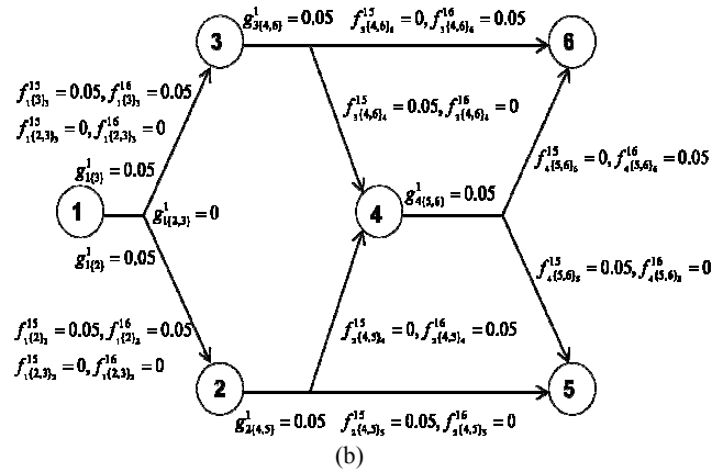
Fig. 2 Numerical example: (a) the wireless butterfly adopted, where the six hyperlinks under consideration are (1, \{2\}) , (1, \{3\}) , (1, \{2, 3\}) , (2, \{4, 5\}) , (3, \{4, 6\}) and (4, \{5, 6\}) (b) the results of g_{ij}^s and f_{ij}^{st} in the example, where each hyperlink with multicast from s = 1 to t \in T_s = \{5, 6\} is marked with g_{ij}^1 and the pair (f_{ij}^{15}, f_{ij}^{16})
