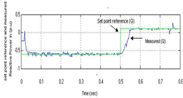
Fig. 17 Reactive power flow over the transmission line for case (b)
