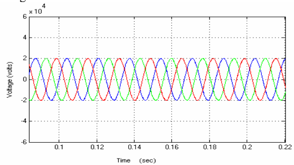
Fig. 7 48-Pulse VSI output voltage for case (a)
