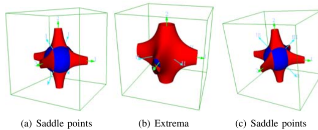
Fig. 7. Saddle points and Extrema obtained by Octave.
