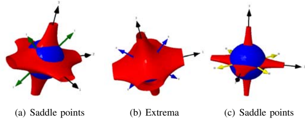
Fig. 4. Saddle points and Extrema obtained by Sage.
