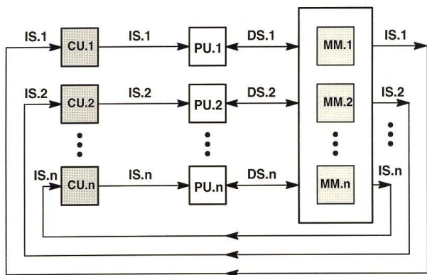
Fig. 1 (c) MIMD computer
