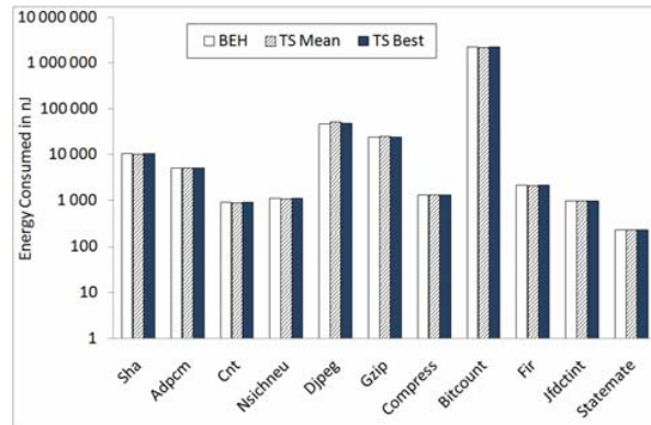
Fig. 2. Energy consumed in standard benchmarks with WB mode.
