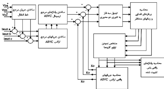
Fig. 4 Diagram block
