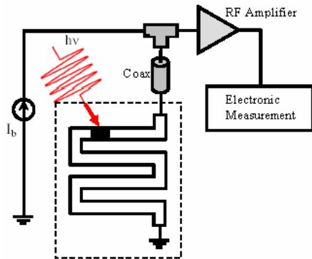
Fig. 3 Driving and measurement circuit
