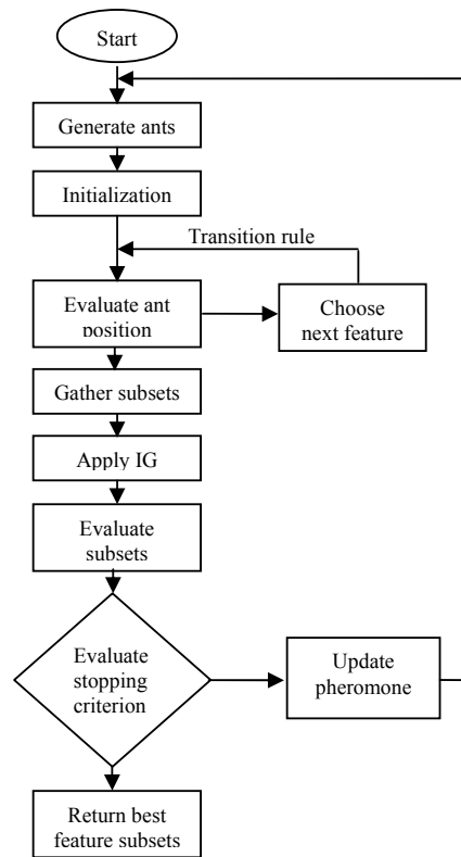
Fig. 3 Flow diagram of ACO-IG feature selection
