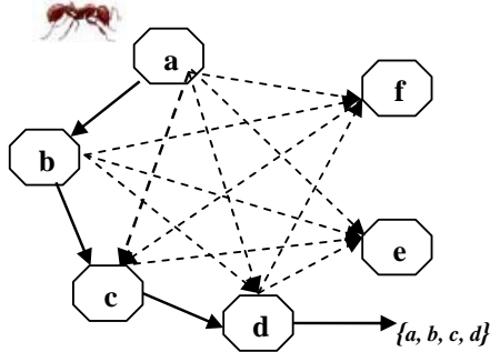
Fig. 1 ACO representation for FS problem
