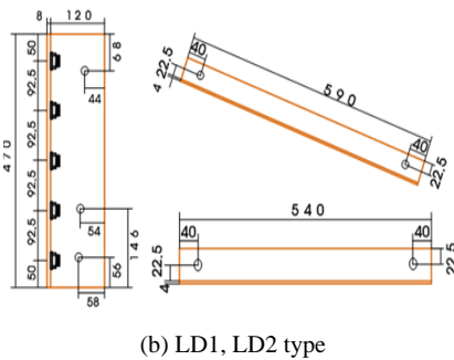
Fig. 4 Detail of Each Specimen
