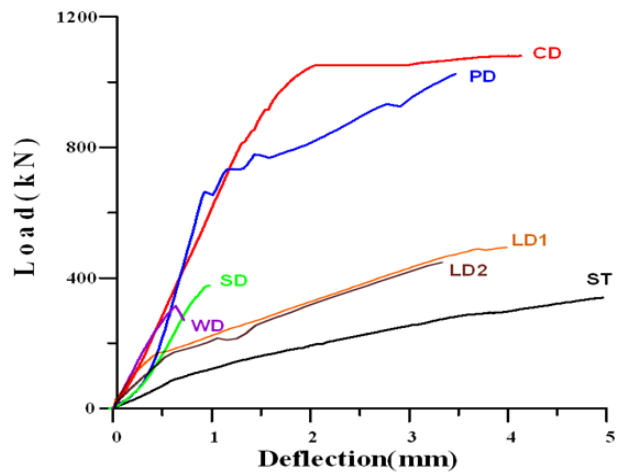
Fig. 7 Load-Deflection Curve at LVDT
