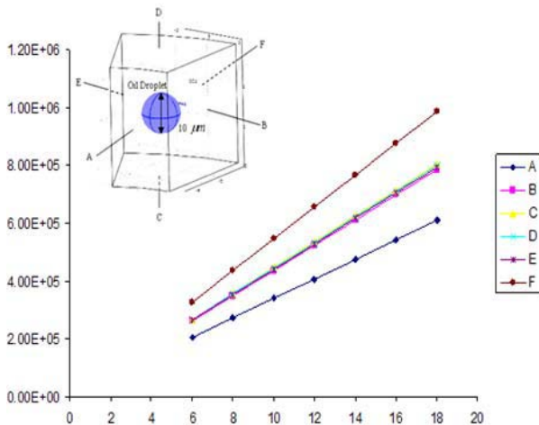
Fig. 4 Local pressure on each boundary of the domain surrounding the 10- \mu m oil droplet
