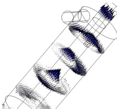
Fig. 9 Vertical velocity distribution on various cross-sections illustrated the fluctuation of the Locus of Zero Vertical Velocity or LZVV due to turbulence
