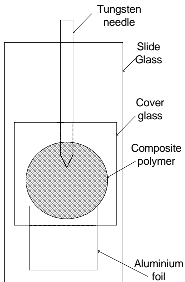
Fig. 2 Configuration of leaf-like specimen
