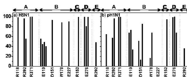
Fig. 3 Percent occupation pattern of hydrogen bonds formed from (A) carboxylate, (B) guanidinium, (C) N-acetyl, (D) trihydroxypropyl, and (E) dihydropyran ring of laninamivir interacting with the NA residues of the two viruses: a) H5N1 and b) pH1N1
