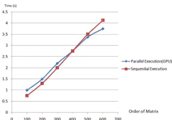
Fig. 19. Performance Monitoring in GPU based Parallelism
