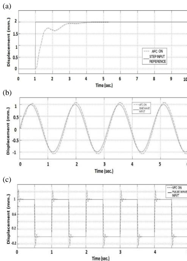
Fig. 9 Effect of harmonic disturbance on system response for PID controller only (AFCFL – ON) for various input conditions
