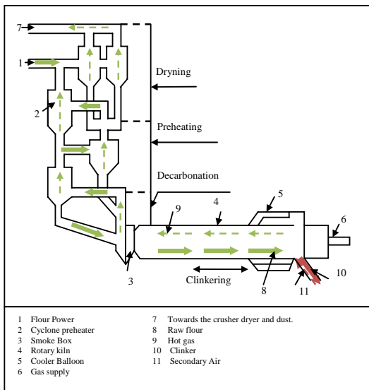
Fig. 8 Flow Diagram of a Rotary Cement Kiln [7]
