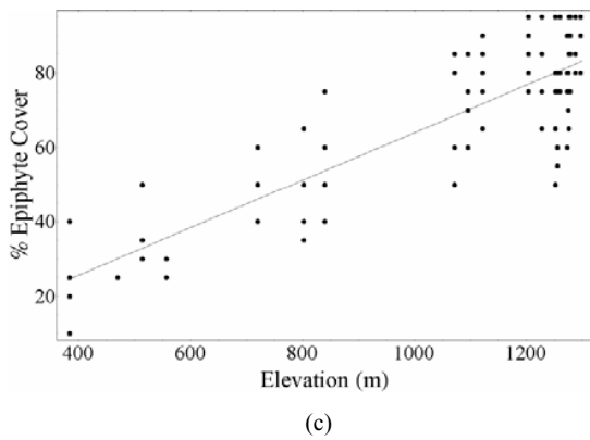
Fig. 4 Vegetation characteristics from Klongkai station to Sanyen cloud forest during 17-21 April 2007. (a) bush height (m) and elevation (m), (b) tree height (m) and elevation (m), and (c) % epiphyte cover and elevation (m)
