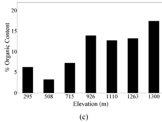
Fig. 5 Soil characteristics and elevation (m) from Klongkai station to Sanyen cloud forest during 17-21 April 2007. Soil characteristics: (a) % soil moisture from field data, (b) % soil moisture from laboratory data and (c) % organic content
