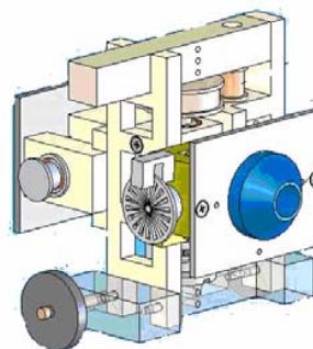
Fig. 12 New Joint design
