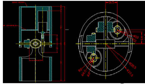
Fig. 15 Assembly plan
