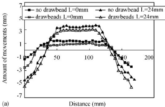
Fig. 7 Comparison of weld line movement of existence of drawbead in Heo et al. investigation [14]
