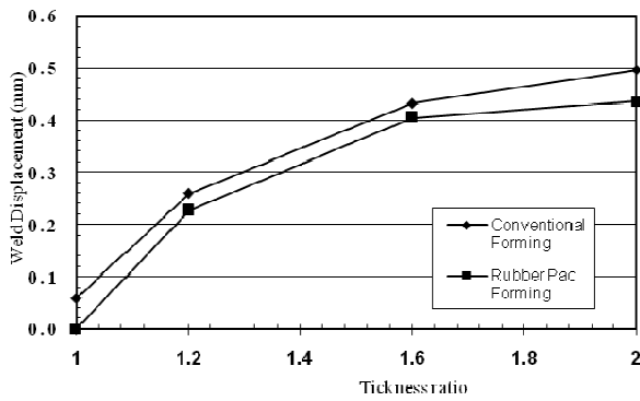
Fig. 5 Experimental weld displacements at failure of difference thickness ratio
