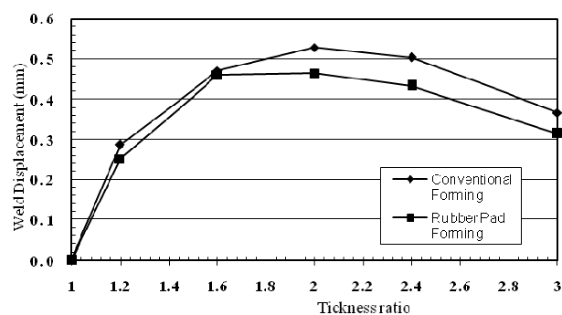
Fig. 4 Weld displacements at failure of difference thickness ratio in numerical results
