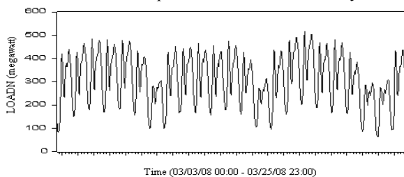
Fig. 4 Hourly load curve of the Italian railways - North Zone of the GME
