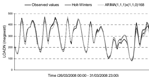
Fig. 8 Forecasts of the hourly load curve of the Italian railways
