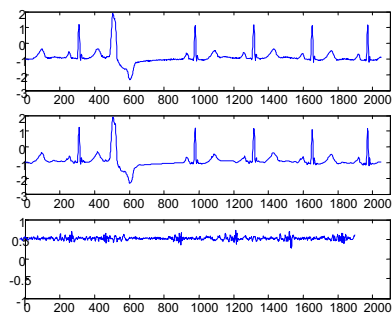
Fig. 4 – Compressing ECG using the cardbal2 with Id prefiltering method. The above figure shows the original signal, the middle shows reconstructed signal after compression and the bottom shows error between them. The first 2048 samples of MIT-BIH record 119 are used. CR=16.384, PRD=4.0136%, CC=99.6335%, D=0.0016109, RMSE=0.039487, SNR=21.3 (dB) RMSE=0.069803, SNR=21.6 (dB)
