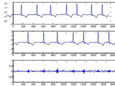
Fig. 5 – Compressing ECG using the cardbal2 with Id prefiltering method. The above figure shows the original signal, the middle shows reconstructed signal after compression and the bottom shows error between them. The first 2048 samples of MIT-BIH record 219 are used. CR=16.384, PRD=5.774%, CC=99.5286%, D=0.0033339, RMSE=0.043508, SNR=20.2 (dB)
