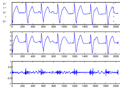
Fig. 3 – Compressing ECG using the cardbal2 with Id prefiltering method. The above figure shows the original signal, the middle shows reconstructed signal after compression and the bottom shows error between them. The first 2048 samples of MIT-BIH record 107 are used. CR=16.384, PRD=7.8842%, CC=99.6612%, D=0.006216.
