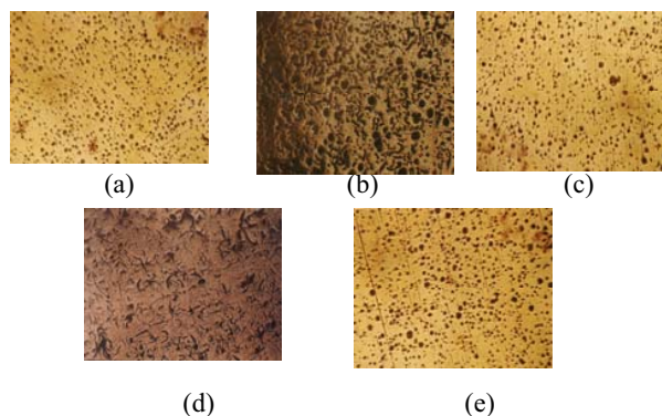
Figure 11 Microstructures of ductile irons before etching ( \times 100 ) by varying weight percentage of magnesium ferrosilicon added when the sizes of magnesium ferrosilicon added are kept constant at 10 mm and the choke and runner across the reaction chamber is not on a straight line and the reaction chamber is cylinder (a) 0.5 % MgFeSi added, (b) 0.75 % MgFeSi added, (c) 1.0 % MgFeSi added, (d) 1.25 % MgFeSi added and (e) 1.5 % MgFeSi added
