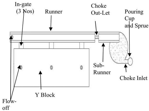
Figure 3 (a) Photograph and (b) drawing for typical gating system of Y-block test specimen. (the choke and runner across the reaction chamber is not on a straight line and the reaction chamber is cylinder)
