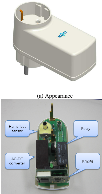
(a) Appearance (b) Configuration Fig. 2 Wireless plug
