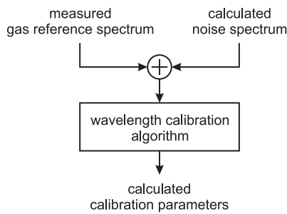
Fig. 3 Block diagram of noise performance simulation
