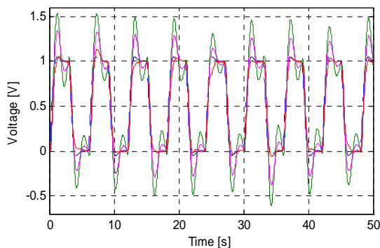
Fig. 11 Time responses of motor voltage on the pulse sequence: PI control without delay (---) and with delay (—), predictive control (—) and predictive control with adaptation delay (—). Average value of time delay is 9 \cdot T
