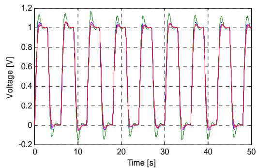
Fig. 9 Time responses of motor voltage on the pulse sequence: PI control without delay (---) and with delay (—), predictive control (---) and predictive control with adaptation delay (—). Average value of time delay is 3*T
