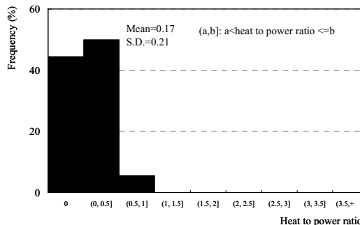
(f) Heat to power ratio in commercial buildings
