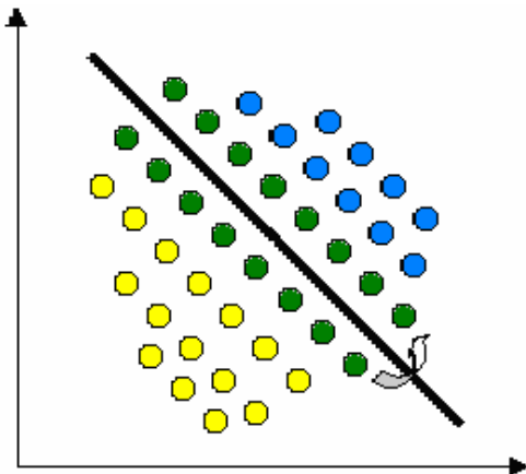
Fig. 2 Overlapping Clustering
