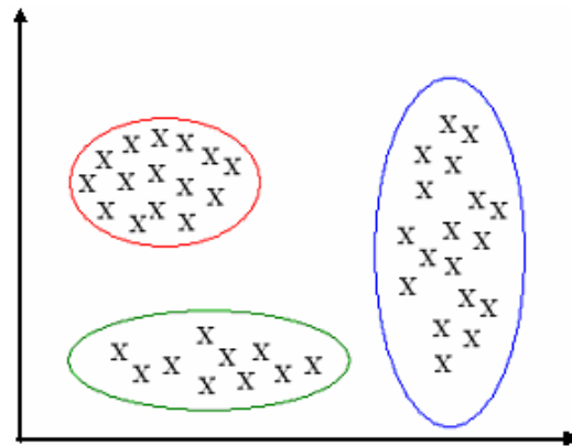
Fig. 1 Clustering
