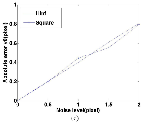
Fig. 4 Accuracy of two methods concerning the noise level
