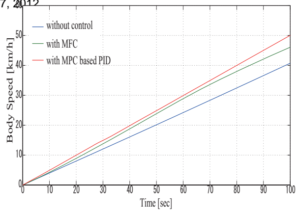
Fig. 8. Vehicl velocity
