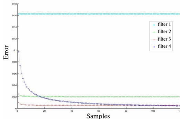
Fig. 7 Interpolation error for limited sequences
