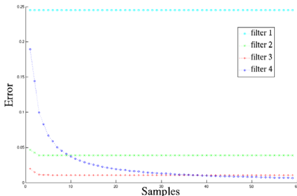
Fig. 8 Interpolation error for limited basis functions
