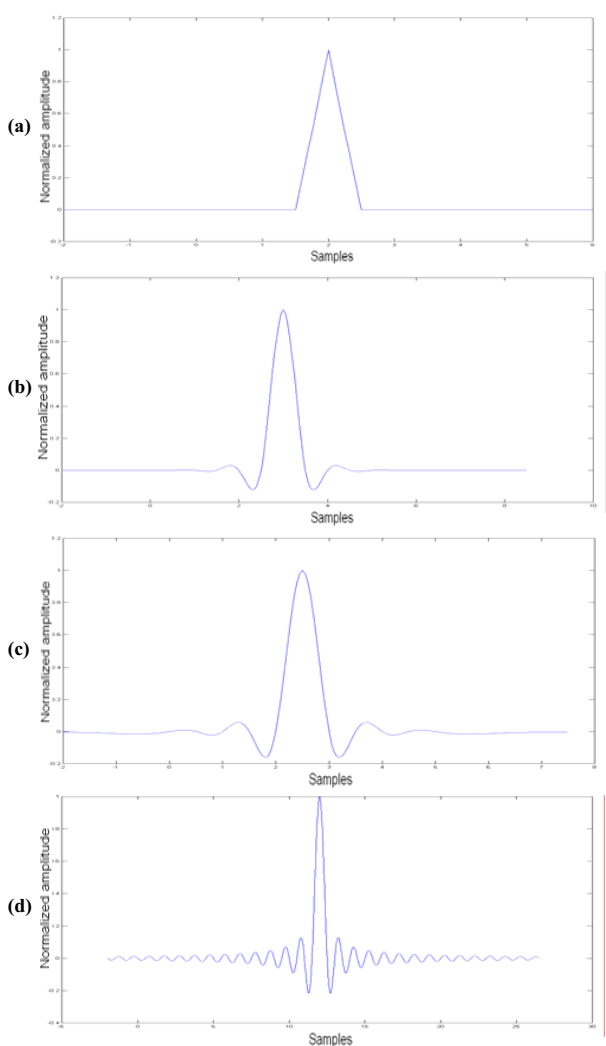
Fig. 3 Basis functions B_j , for different low pass filters. (a) Filter 1. (b) Filter 2. (c) Filter 3. (d) Ideal filter (truncated sinc(t) )
