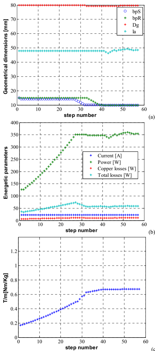
Fig. 4. The parameters evolution in the optimization process of SRM.
