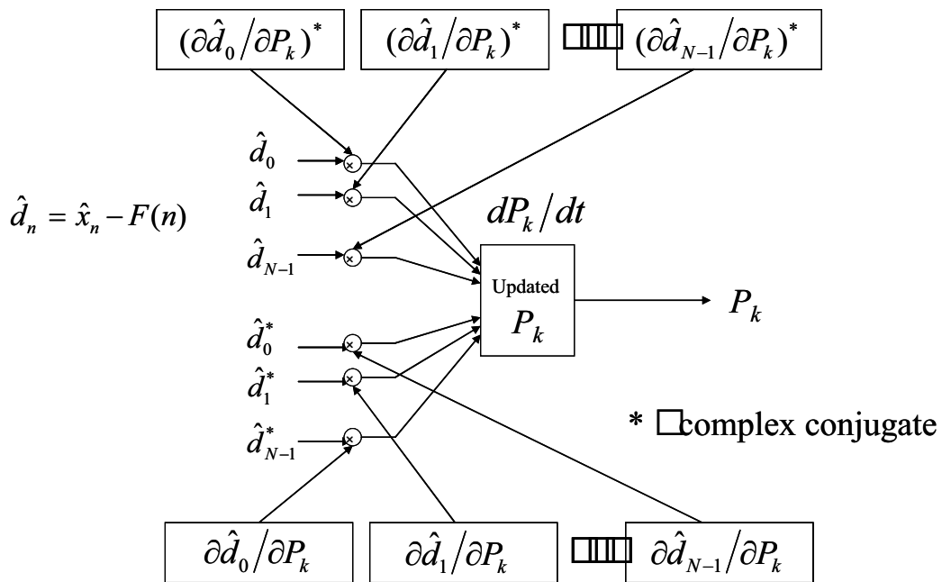
Fig. 1 Structure of the modified Hopfield neural network
