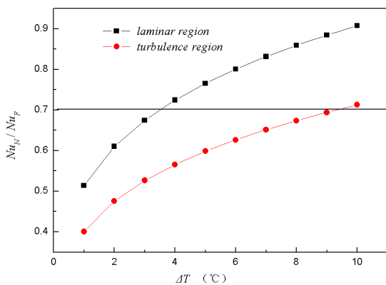
Fig. 5 Nu_N/Nu_F of air flow with 0.6m/s velocity
