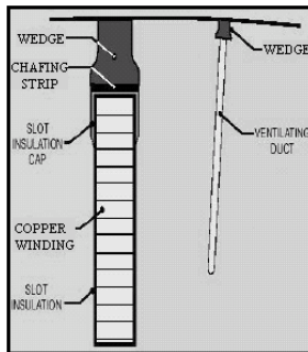
Fig. 1 Indirect cooled coil slot.
