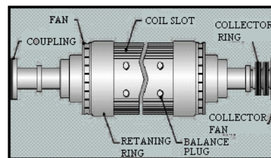
Fig. 3 Generator field
