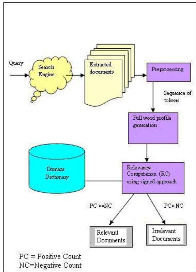
Fig. 1 Architectural Design of the proposed System
