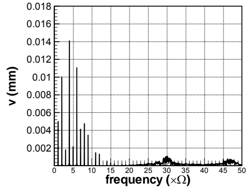
Fig. 11 The response spectra at the end point E of the follower undergoing 3-4-5 polynomial motion for \Omega = 240 rad/s.
