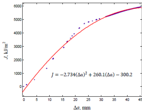
Fig. 10 Monotonic J-R curve for specimen SSPW12-27
