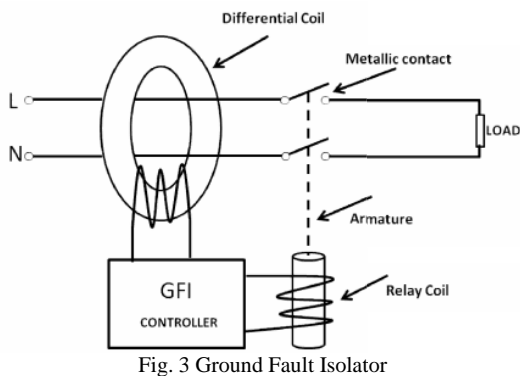
Fig. 3 Ground Fault Isolator
