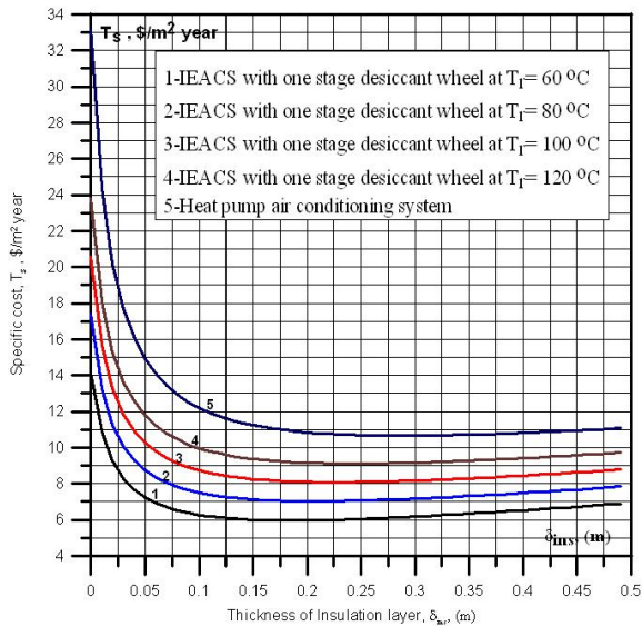
Fig. 14. Specific costs T_s, \$/m^2 per year, for IEACS with one stage of desiccant wheel system for conditions of Egypt, city Aswan depending on the thickness \delta_{ins} , m of the building envelope.
