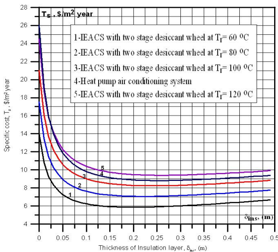
Fig. 15. Specific costs T_s, \$/m^2 per year, for IEACS with two stage of desiccant wheel system for the conditions of Egypt, city Cairo depending on the thickness \delta_{ins} , m of the building envelope.
