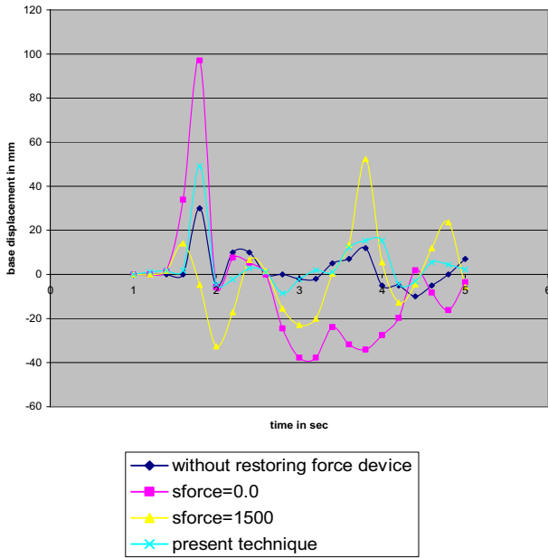
Fig. 5(a) Variation of displacement with frequency
