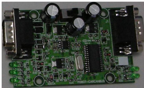
Fig. 5 OBD-II to RS232 adapter
