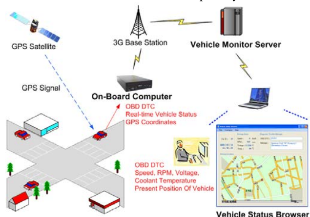
Fig. 2 Configuration of remote on-line diagnostic system
