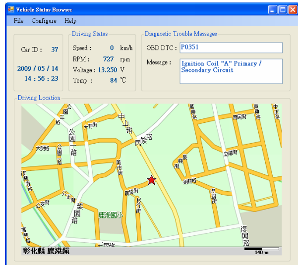
Fig. 11 Vehicle status browser
