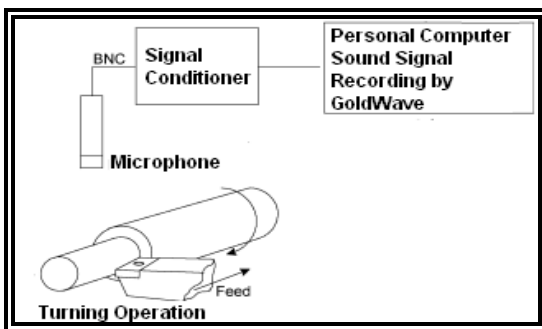
Fig. 2 The tool wears data collection arrangement.
