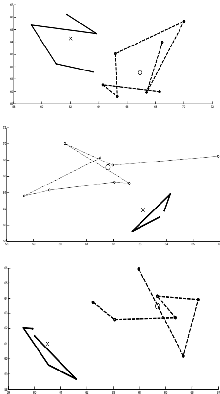
Fig. 4 Fuzzy clustering of tool bit sounds. a) Fresh and slightly worn, b) Slight and severely worn, c) Fresh and severely worn (1 Second High speed signals , Aluminium Job)
