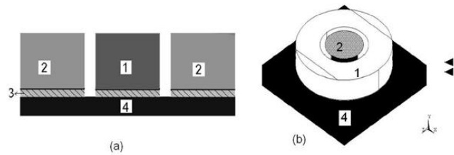
Fig. 2 The schematic diagram the tactile sensor showing a) the cross sectional and b) the three
