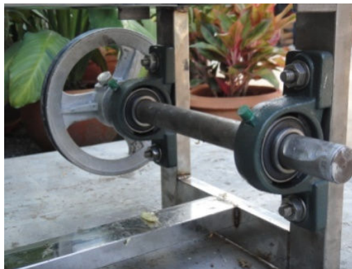
Fig. 13 The pulley and shaft
