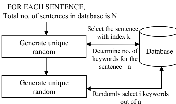
Fig. 3 Generation of Session Parameters
