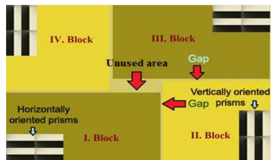
Fig. 3 Steudls algorithm [7]
