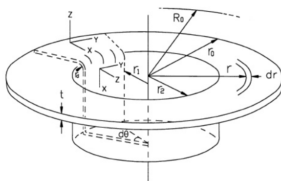
Fig.1 Schematic of deep drawing process
