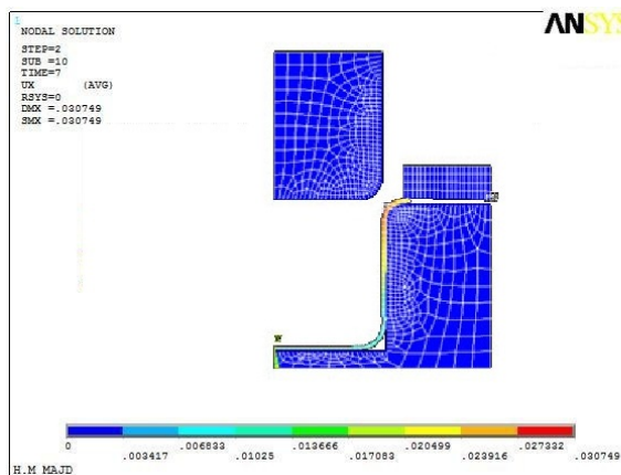
Fig.2 FEM simulation
